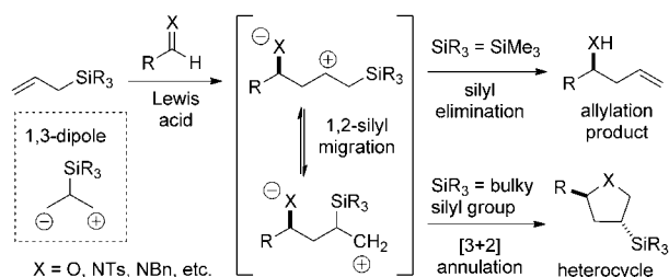
Scheme 1. Mechanism of allylation versus annulation pathways. Bn = benzyl, Ts = 4-toluenesulfonyl.
